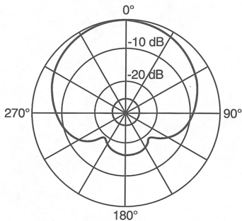
Polar Response (Measured at 1 kHz)
