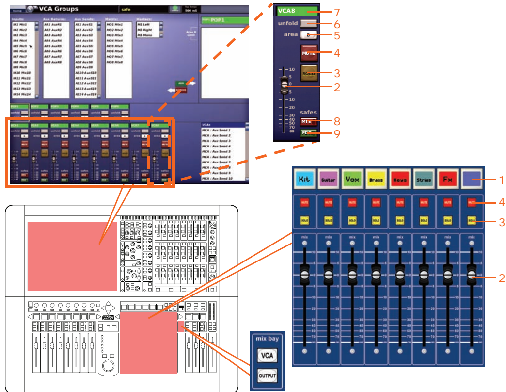
VCA groups on the control surface and GUI
