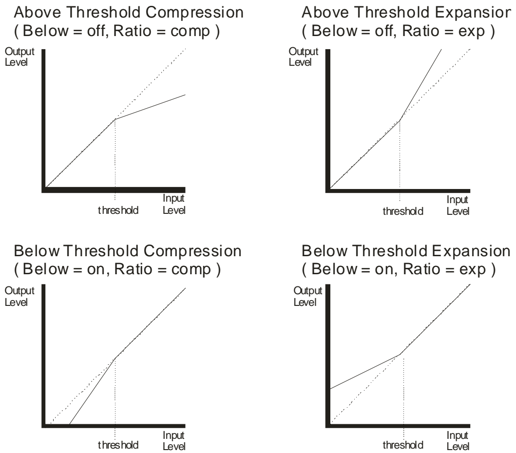
Figure 10: Transfer characteristics
