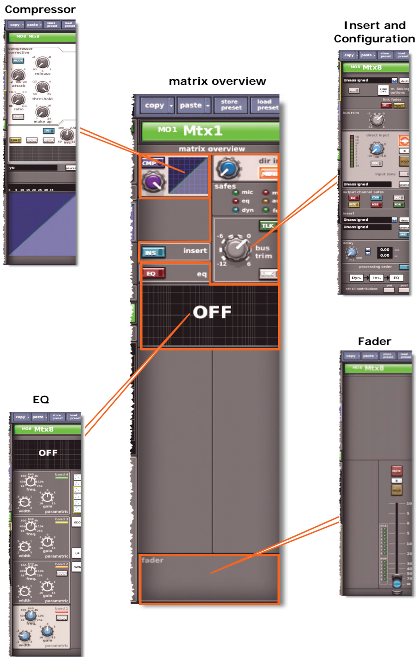
Figure 26: Processing areas available from the matrix overview display
