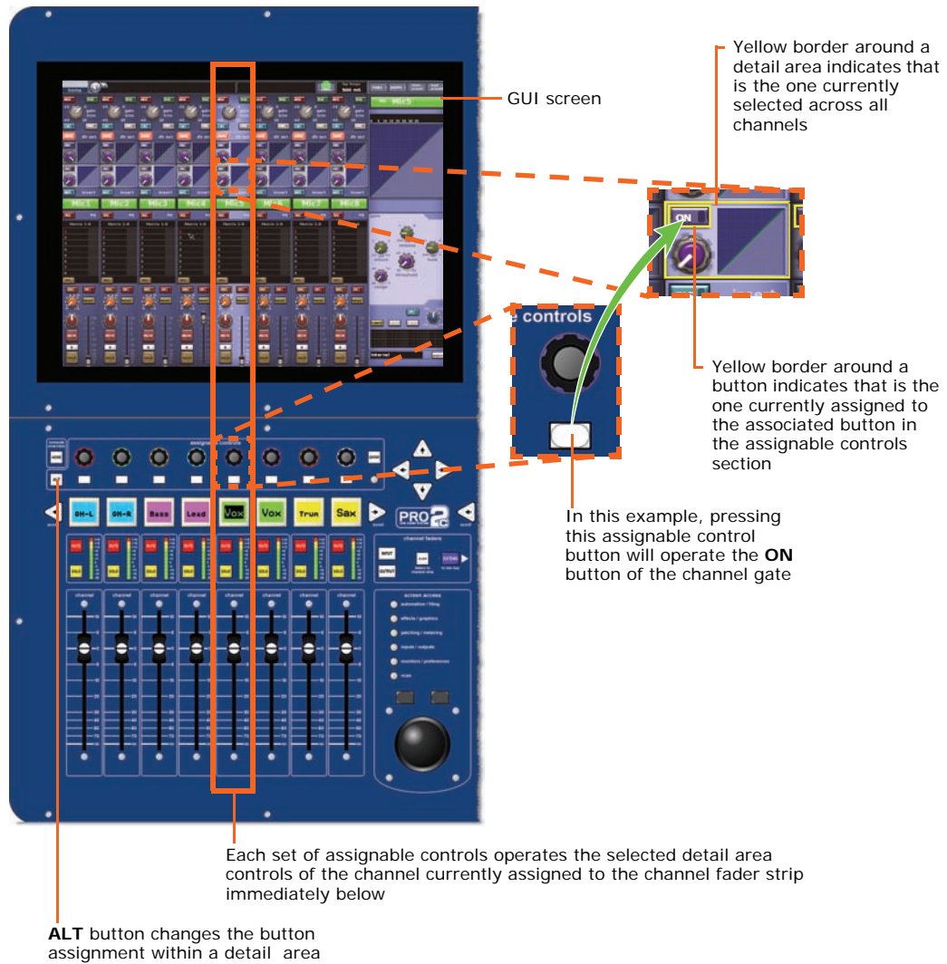
Diagram showing the detail area control assignments of the assignment controls
