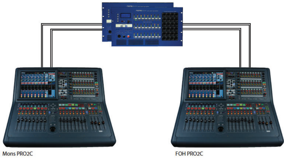
Dual PRO2C FOH and MON system using XL8 DL431 input splitters
