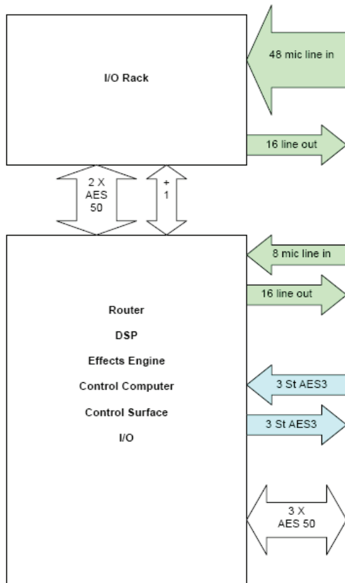
Basic interconnectivity of a standard PRO2 Live Audio System
