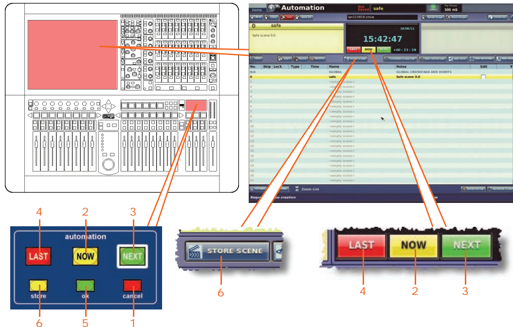
Automation controls on the control surface and GUI
