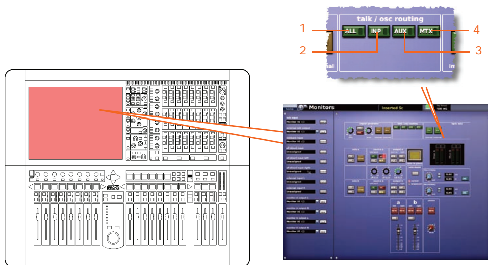
Talk osc/routing controls on the control surface and GUI
