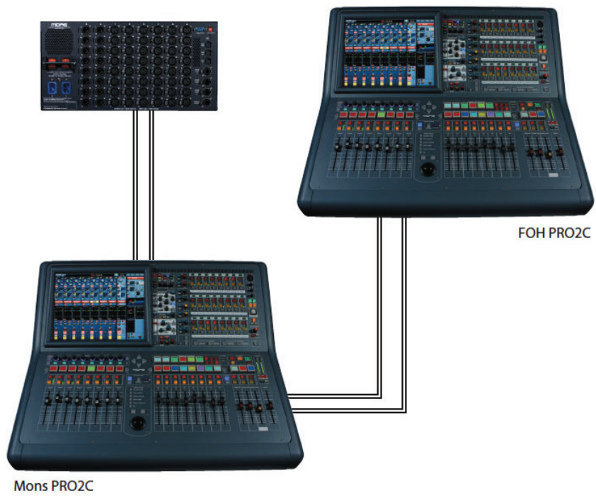
Dual PRO2C FOH and MON system using a DL251 split network
