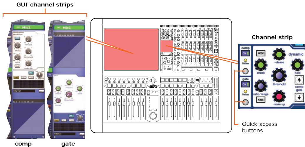
Figure 5: Compressor and gate channel strips
