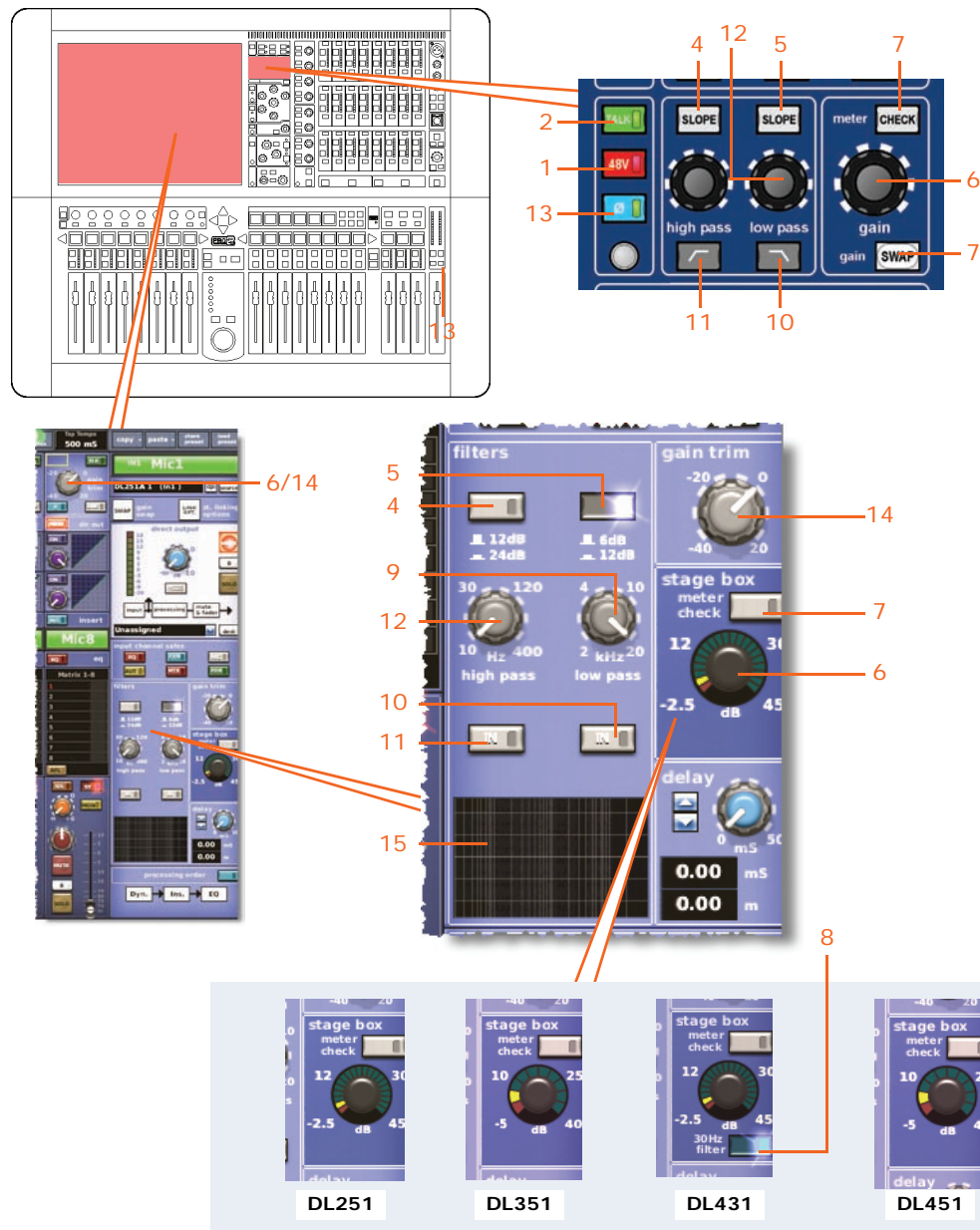
Mic amp input gain on the control surface and GUI
