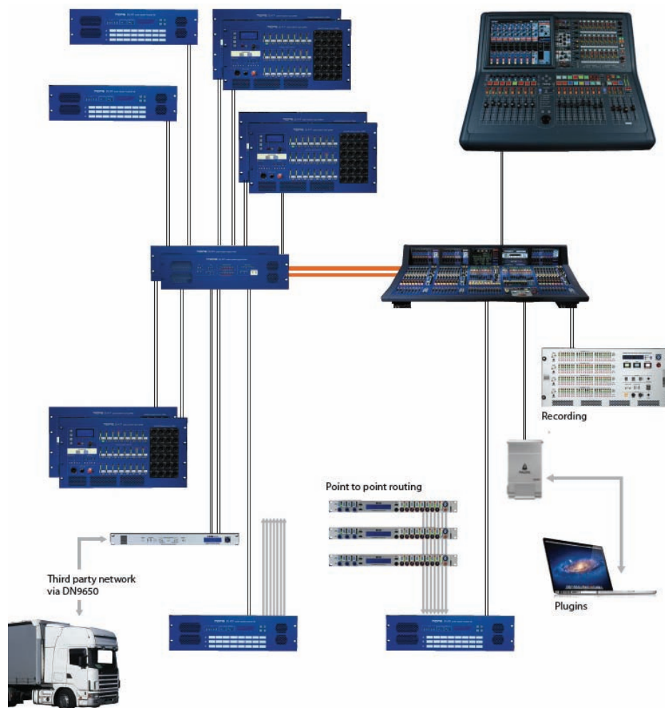
PRO2C and XL8 sidecar network with up to 576 inputs and up to 224 simultaneous channels. The PRO2C control centre and engine are connected to the XL8 network as an extender. The channel count depends upon the number of I/Os and their configuration.
