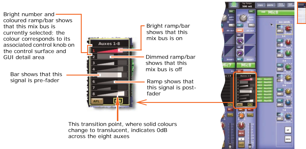
Figure 7: Typical mix section in a GUI input fast strip
