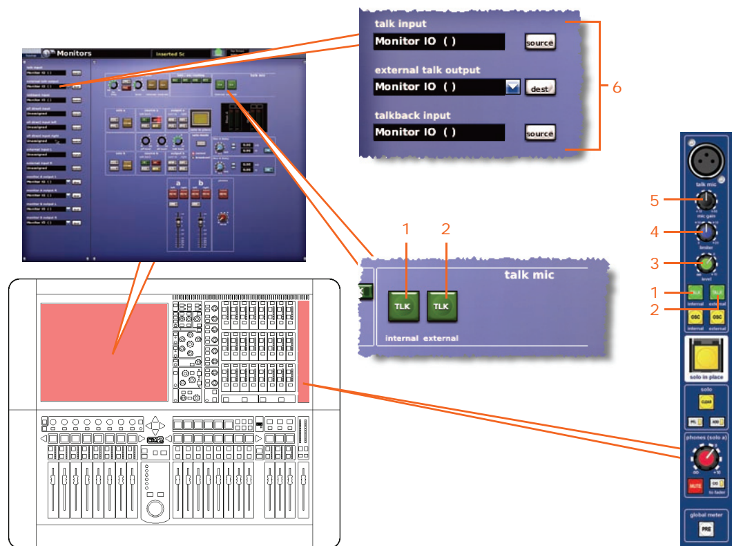
Talk mic controls on the control surface and GUI
