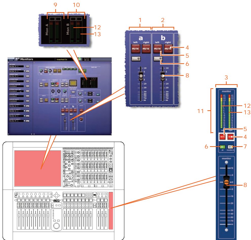
Figure 9: Monitor A and B strips
