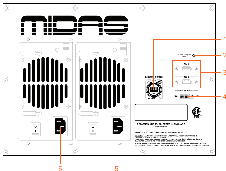
External connections on the right rear panel of the control centre
