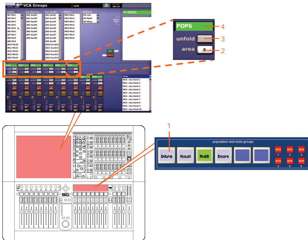
POPulation groups on the control surface and GUI
