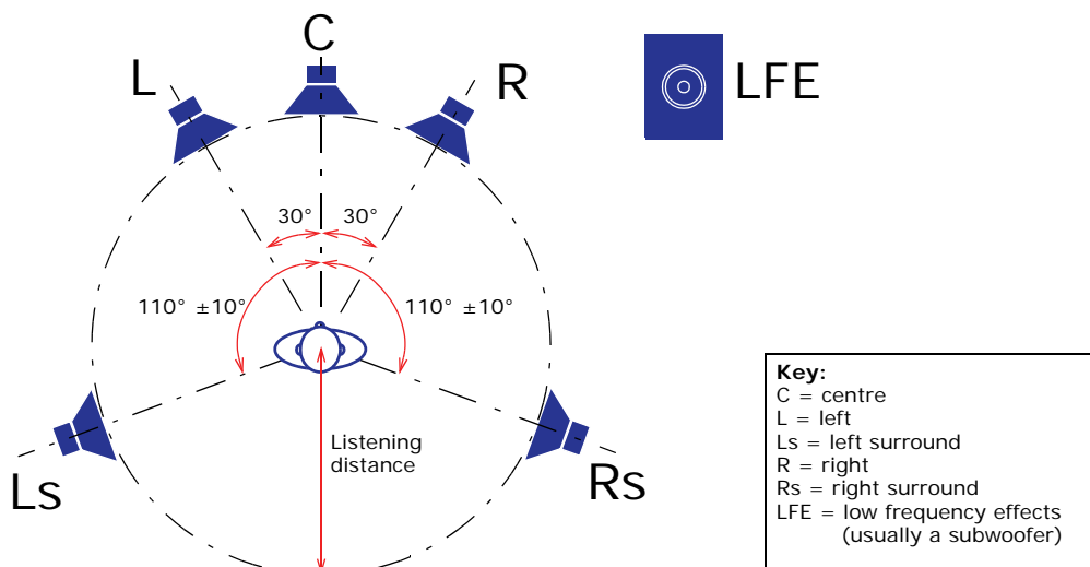
Figure 8: 5.1 surround panning loudspeaker arrangement
